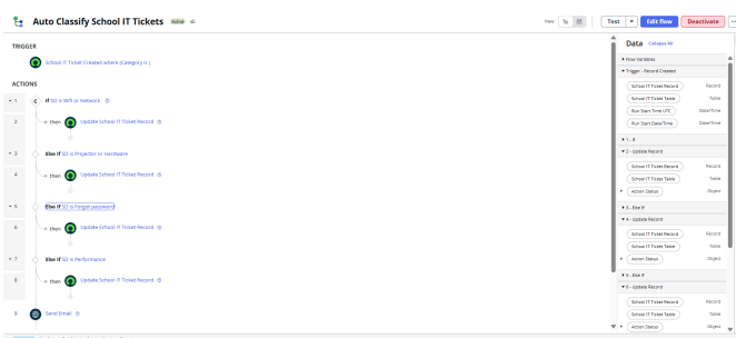
Figure 2: Published Auto Classify School IT Tickets flow.
