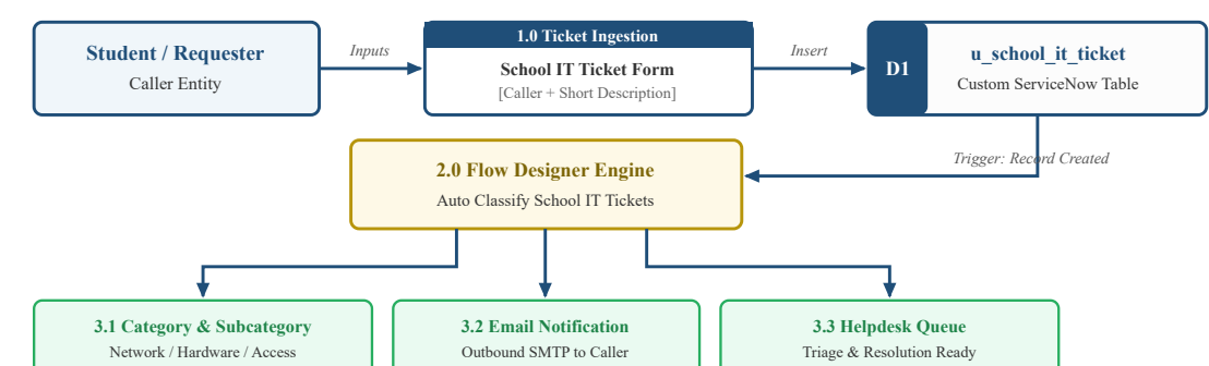
Figure 1: Data flow for the automatic classification process.
